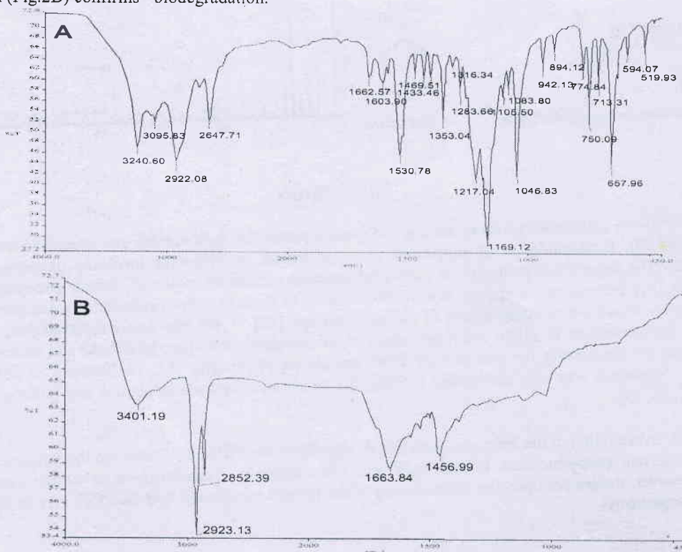
Fig.2A. FTIR spectrum of control 1 Amino 2 naphthol 4 sulphonic acid, 2B. FTIR spectrum of metabolites obtained after degradation of 1 Amino 2 naphthol 4 sulphonic acid.
